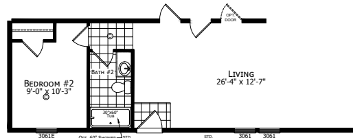
2 BEDROOM OPTION
